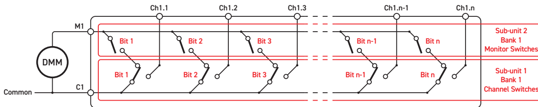
40-619 1-Pole Multiplexer With Monitor - Architecture Showing Monitor Bus Usage
