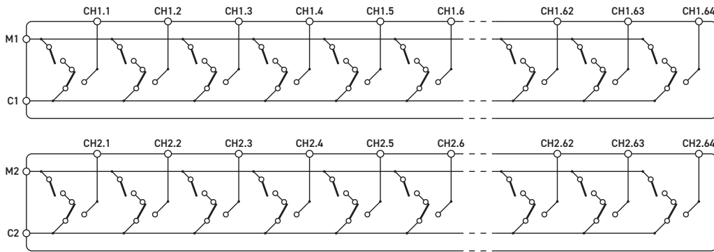
40-619-302 Dual 64-Channel 1-Pole Multiplexer With Monitor
