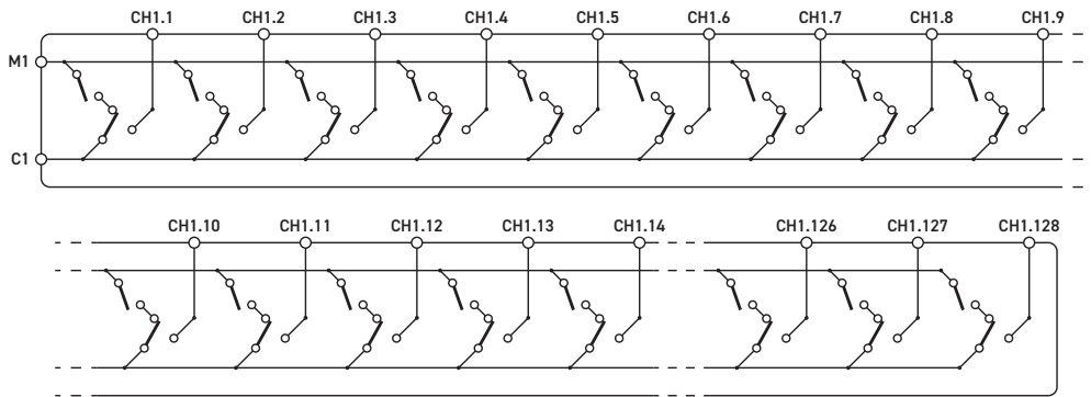
40-619-401 Single 128-Channel 1-Pole Multiplexer With Monitor
