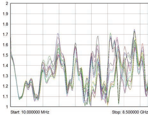
VSWR COM to Channel for 40-883A-002 showing all paths up to 8.5 GHz
