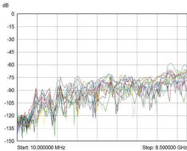
Max isolation for each channel with distant path selected for 40-883A-002 up to 8.5 GHz
