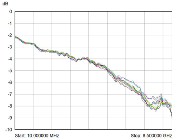
Insertion loss for 40-883A-002 showing all paths up to 8.5 GHz
