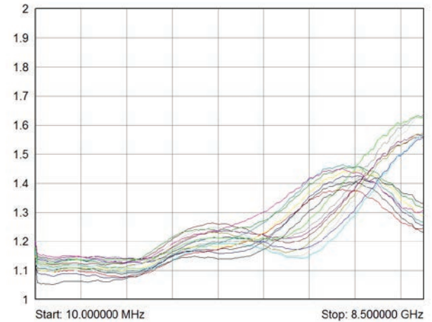
VSWR internal termination on channel for 40-883A-002 showing all paths up to 8.5 GHz
