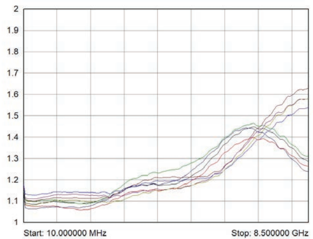
VSWR internal termination on channel for 40-883A-001 showing all paths up to 8.5 GHz
