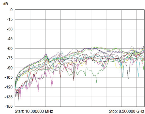
Crosstalk for 40-883A-002 between adjacent channels showing all paths up to 8.5 GHz
