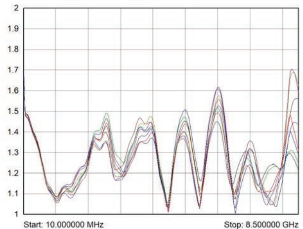
VSWR Channel to COM for 40-883A-001 showing all paths up to 8.5 GHz
