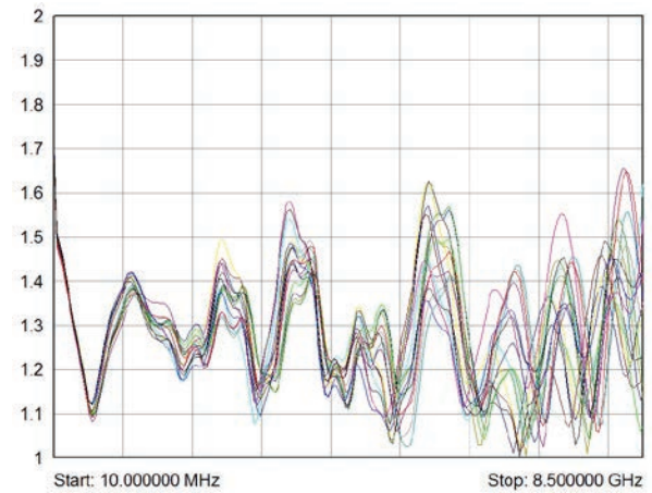
VSWR Channel to COM for 40-883A-002 showing all paths up to 8.5 GHz
