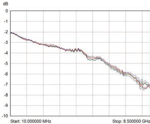
Insertion loss for 40-883A-001 showing all paths up to 8.5 GHz
