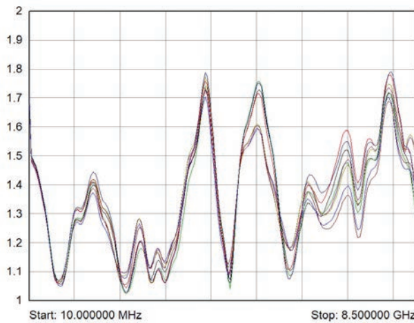
VSWR COM to Channel for 40-883A-001 showing all paths up to 8.5 GHz
