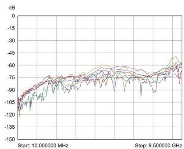
Crosstalk for 40-883A-001 between adjacent channels showing all paths up to 8.5 GHz
