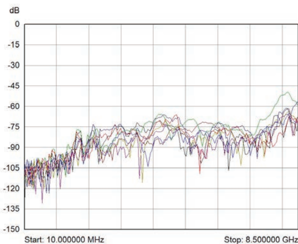
Max isolation for each channel with distant path selected for 40-883A-001 up to 8.5 GHz
