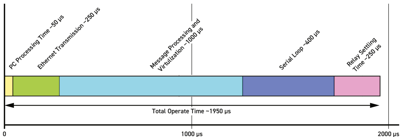
Speed of Operation Diagram For The 65-225
