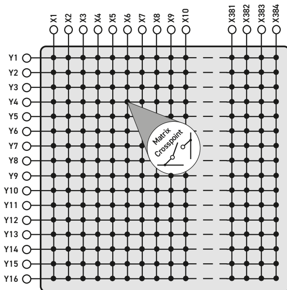
Simplified Diagram For 65-225 Configured as a 384x16 Matrix
